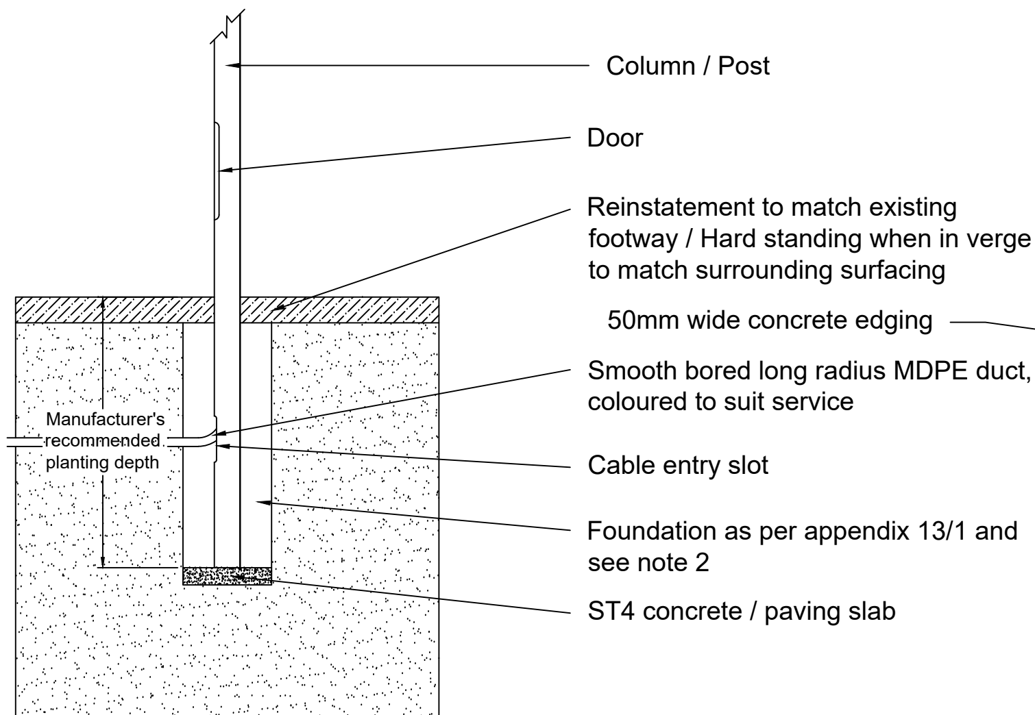
Planted Foundation Elevation
